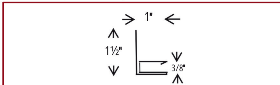
3/8" F-Trim (Aluminum)
